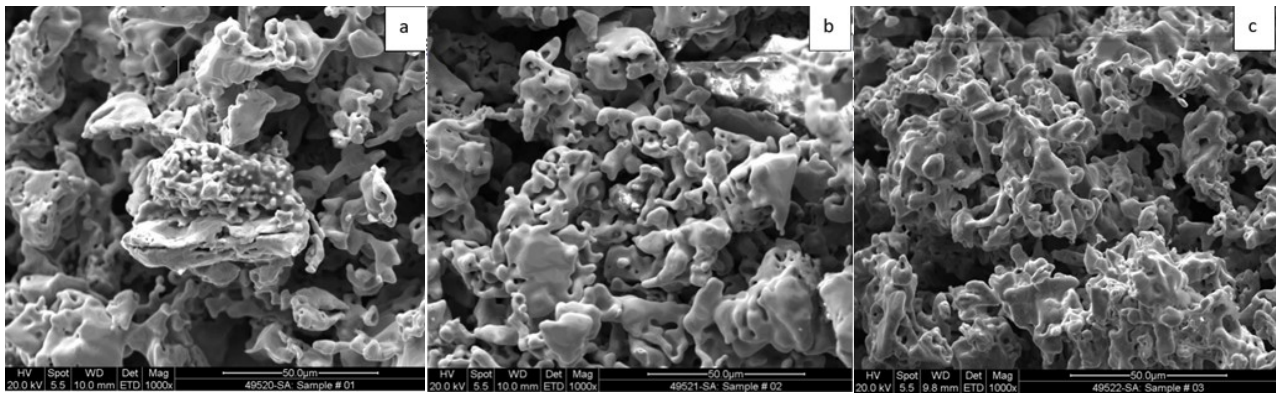
Fig. 9 SEM micrographs of reduced iron ore pellets coated with: 10% steel dust slurry conc. & 3.0 kg per ton iron ore pellets; 10% steel dust slurry conc. & 4.0 kg per ton iron ore pellets; 10% steel dust slurry conc. & 5.0 kg per ton iron ore pellets
