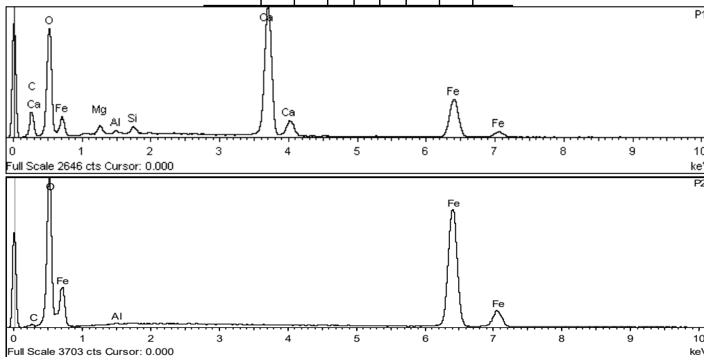
Fig. 7 SEM photo and EDX analysis for lime coating layer of iron ore pellets
