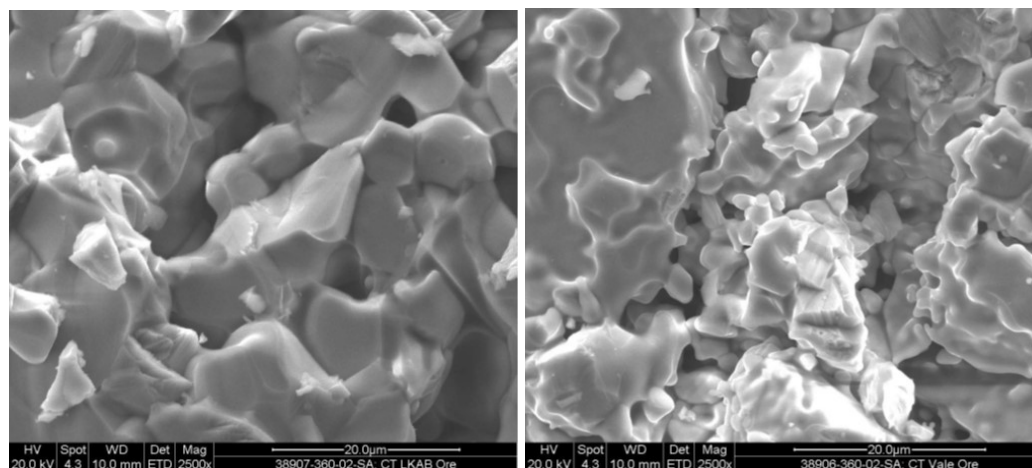
Fig. 5 SEM micrographs of iron ore pellets
