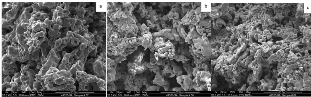
Fig. 13 SEM micrographs of reduced iron ore pellets coated with: (a) 30% steel dust slurry conc. & 3.0 kg per ton iron ore pellets; (b) 30% steel dust slurry conc. & 4.0 kg per ton iron ore pellets; (c) 30% steel dust slurry conc. & 5.0 kg per ton iron ore pellets
