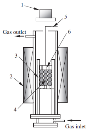
Fig. 1 Schematic diagram of the reduction apparatus 1-Weighting system, 2- Tube furnace, 3- Sample holder, 4- Sample bed in ceramic balls, 5- Thermocouple and 6- Upper arid lower lift
