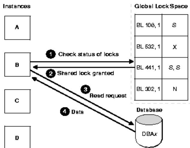
Fig. 1 Locking management in distributed databases
