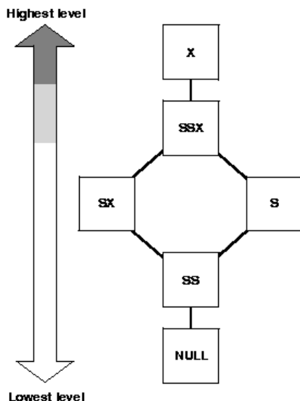
Fig. 2 Two phases locking approach
