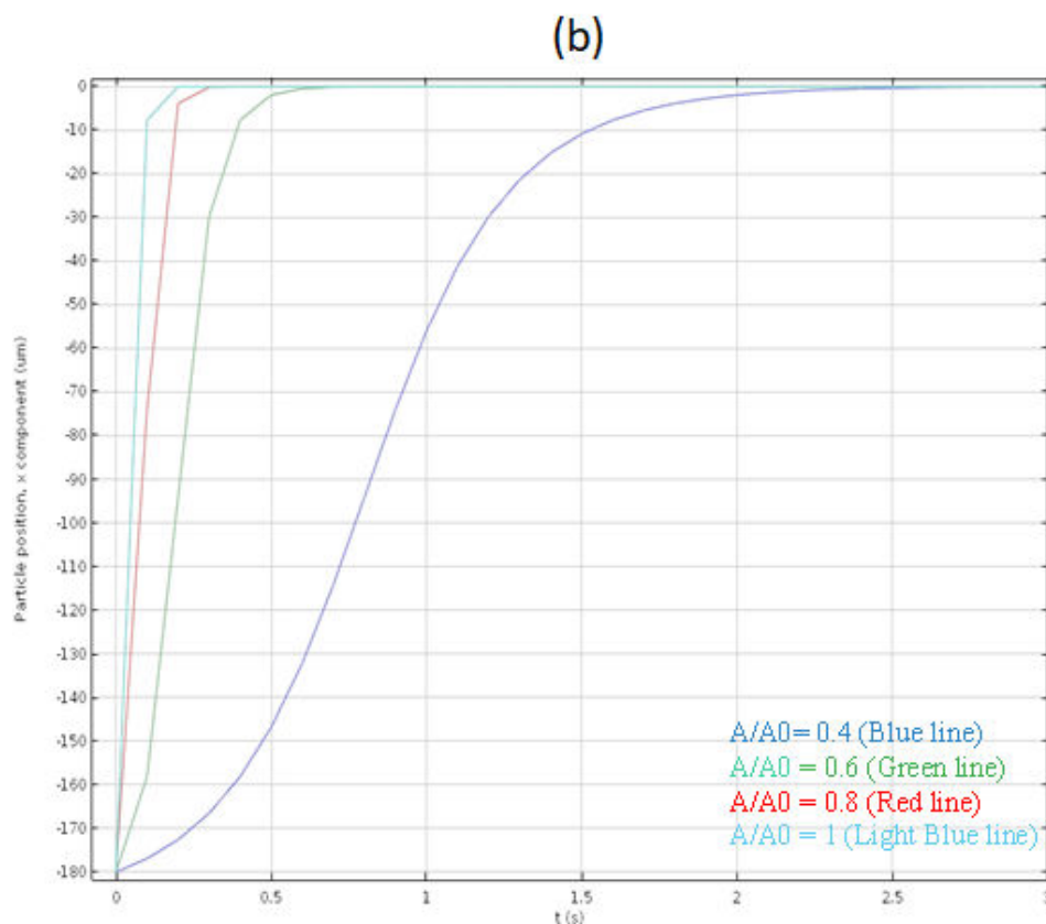
Fig. 5 Particle position versus time for variety of amplitude ratio; (a) particle size equals 1 µm; (b) particle size equals 5 µm
