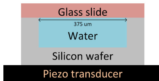
Fig. 1 Depiction of the acoustophoresis device
