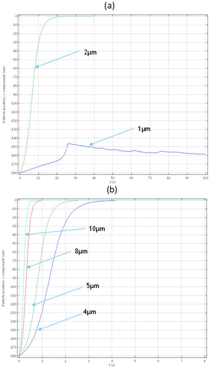
Fig. 2 Particle position versus time; (a) 2 μm and 1 μm; (b) 4 μm, 5 μm, 8 μm and 10 μm
