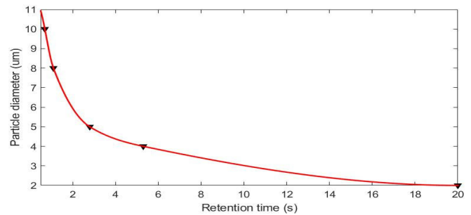
Fig. 3 Particle diameter versus retention time
