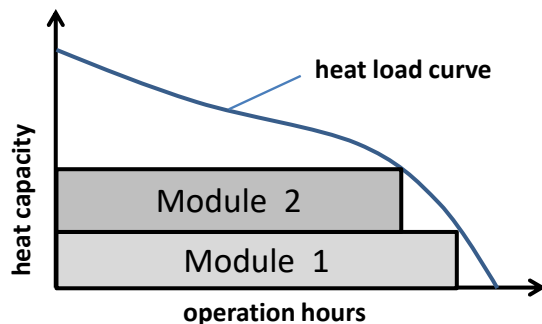
Fig. 7 Heat load curve with CHP modules
