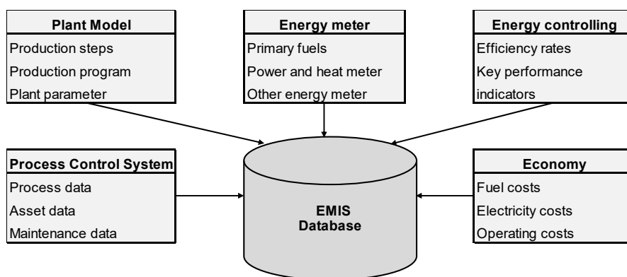
Fig. 3 Energy information system
