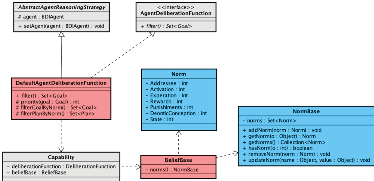
Fig. 4 Deliberative Goals Function
