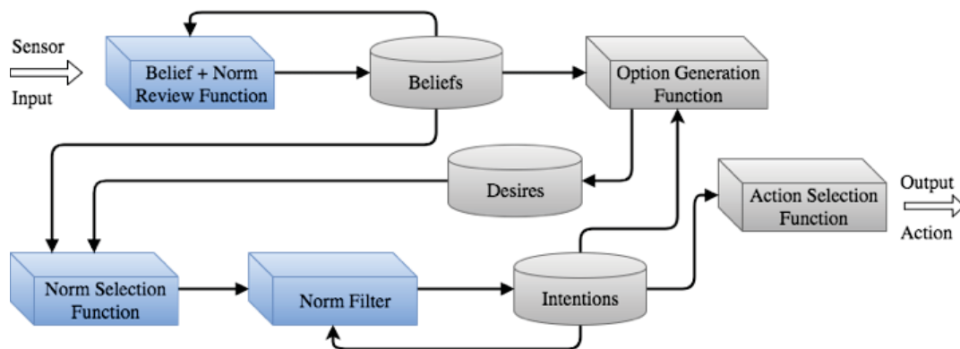
Fig. 1 BDI Architecture + NBDI Architecture
