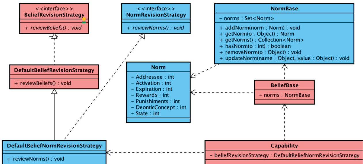
Fig. 3 Revision Norms and Beliefs Function
