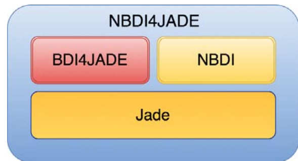
Fig. 2 The NBDI4JADE Architecture
