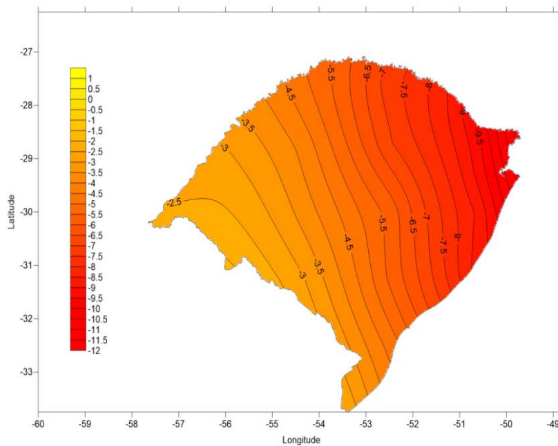
Fig. 6 Averages of solar radiation anomalies kWh / m 2 (%) Scenario 2 (2076 - 2100)
