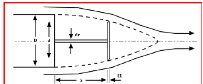
Fig. 2 Locked vortex afterbodies
