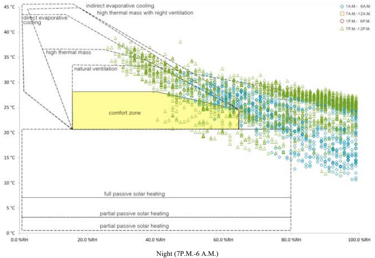
Fig. 5 The relationship between temperature and relative humidity value in thermal comfort chart
