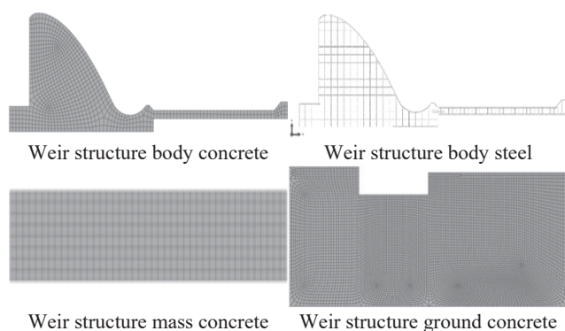
Fig. 4 Modeling of separated part of weir structure
