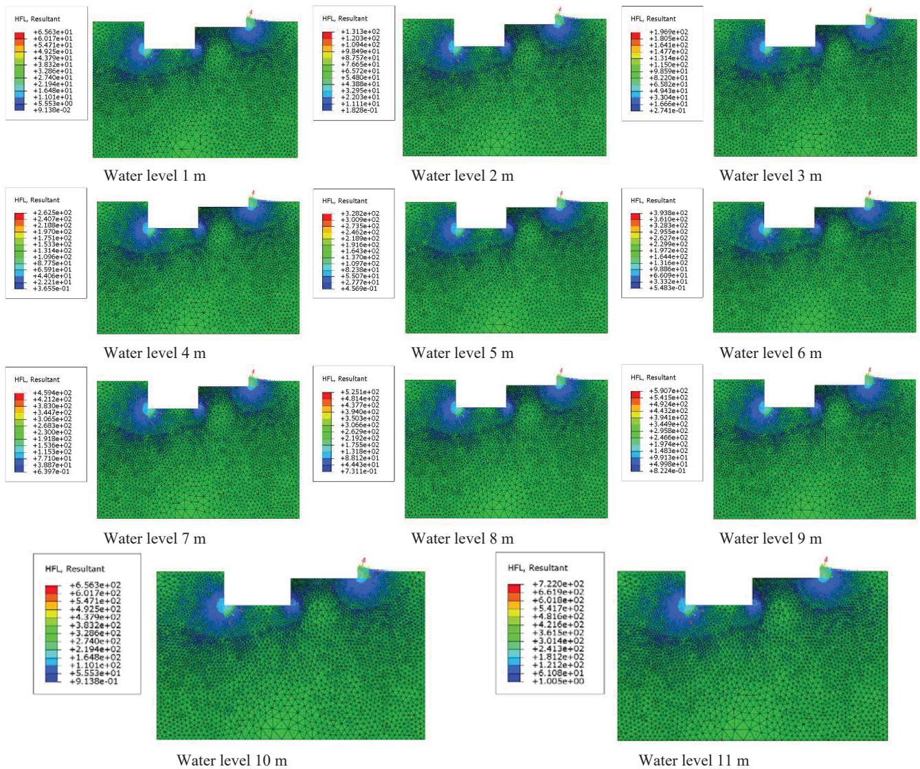
Fig. 8 Contour results of seepage analysis
