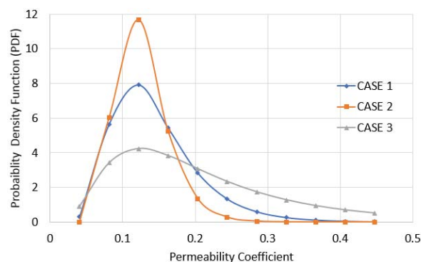
Fig. 7 Permeability coefficients log normal distribution
