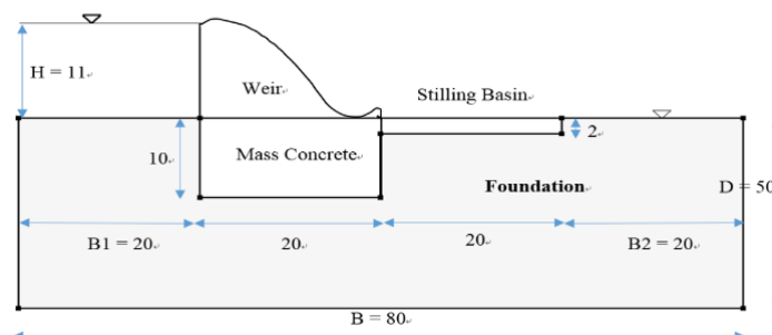
Fig. 3 Weir structure profile and dimensions
