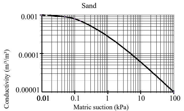
Fig. 3 Conductivity for sand
