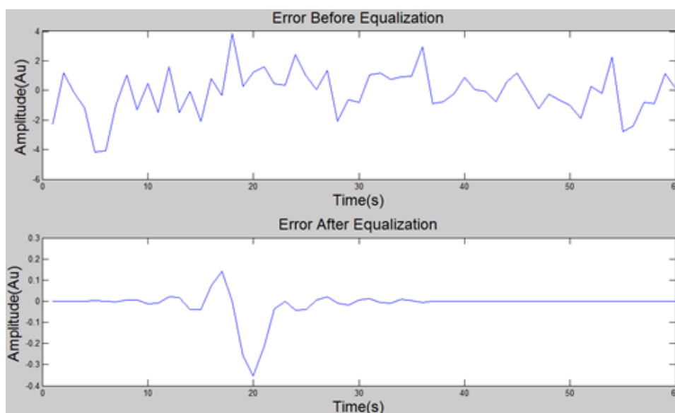
Fig. 12 Comparison of errors before and after equalization
