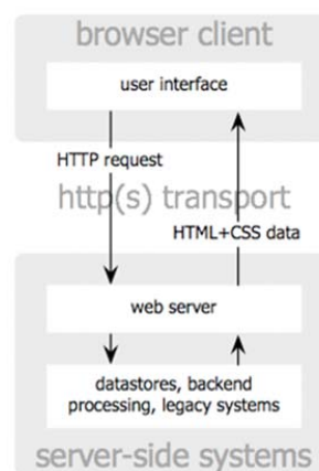
Fig. 1 Client-Server Architecture [1]
