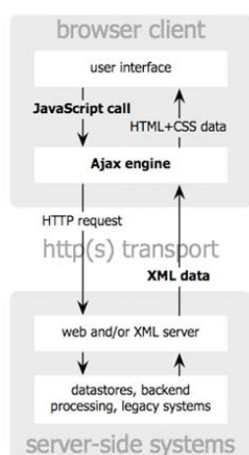
Fig. 2 Client-Side Architecture [1]
