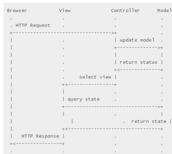
Fig. 3 MVC Architecture [1]
