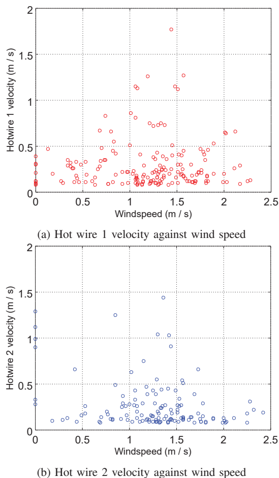
Fig. 9 Hot wire measurements against wind speed for northern sector winds(perpendicular to the test cell face) as obtained from the ultrasonic anemometer. The north wind direction uncertainty was binned on the basis of \pm 10^\circ uncertainty range. Data is 1 minute averaged
