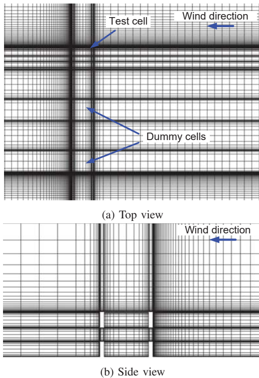
Fig. 6 Mesh details close to the test cell
