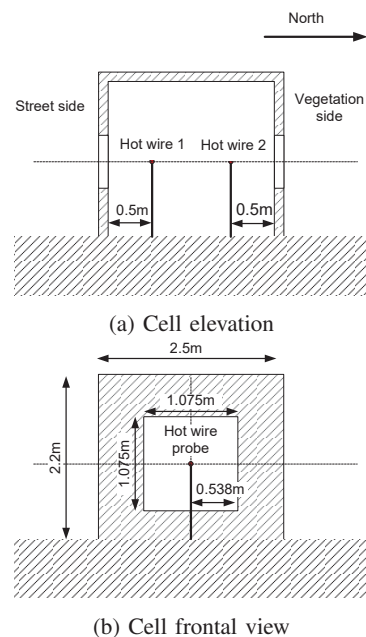
Fig. 2 Cell dimensions and hot wire positions
