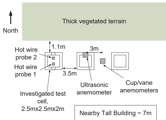
Fig. 1 Top view of setup and critical dimensions.
