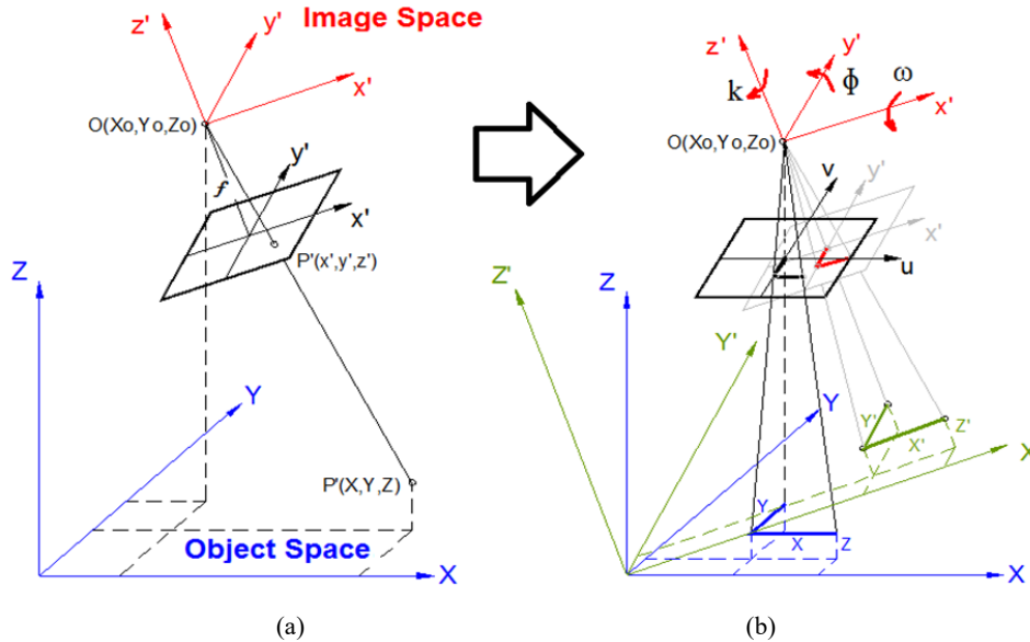
Fig. 1 Collinearity between Object Space and Image Space
