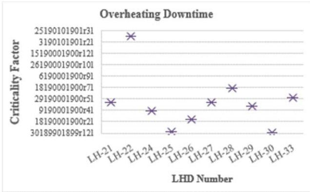
Fig. 4 Criticality Factors of 17 tonnes LHDs for Overheating problem
