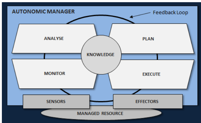
Fig. 2 The Autonomic Manager and MAPE-K feedback loop
