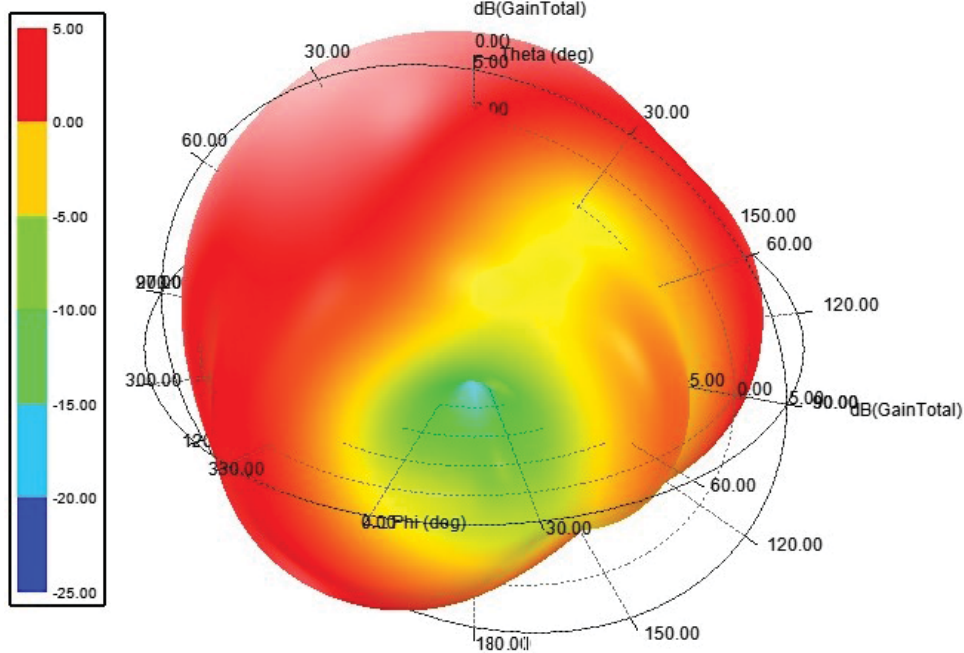
(b) Radiation patterns of antenna 4
