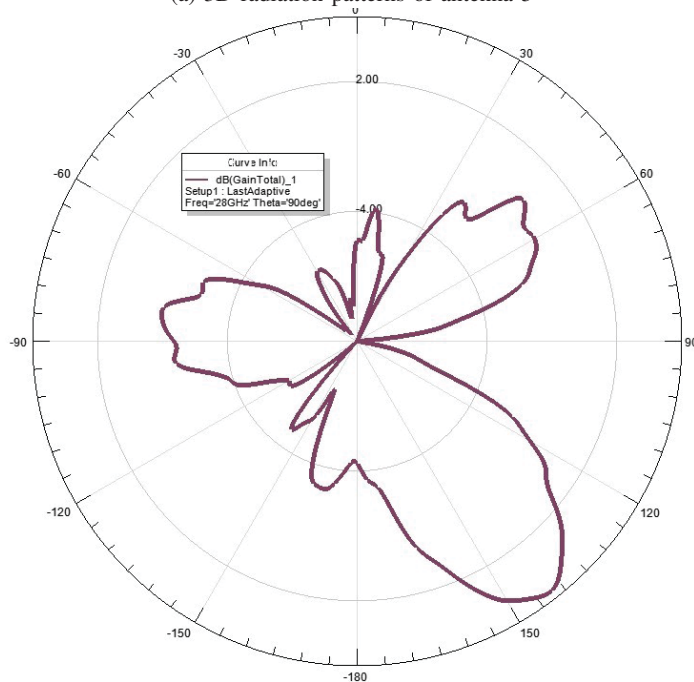
(b) 2D radiation patterns of antenna 5
