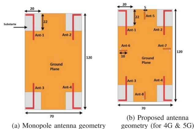
Fig. 1 Geometry of antennas
