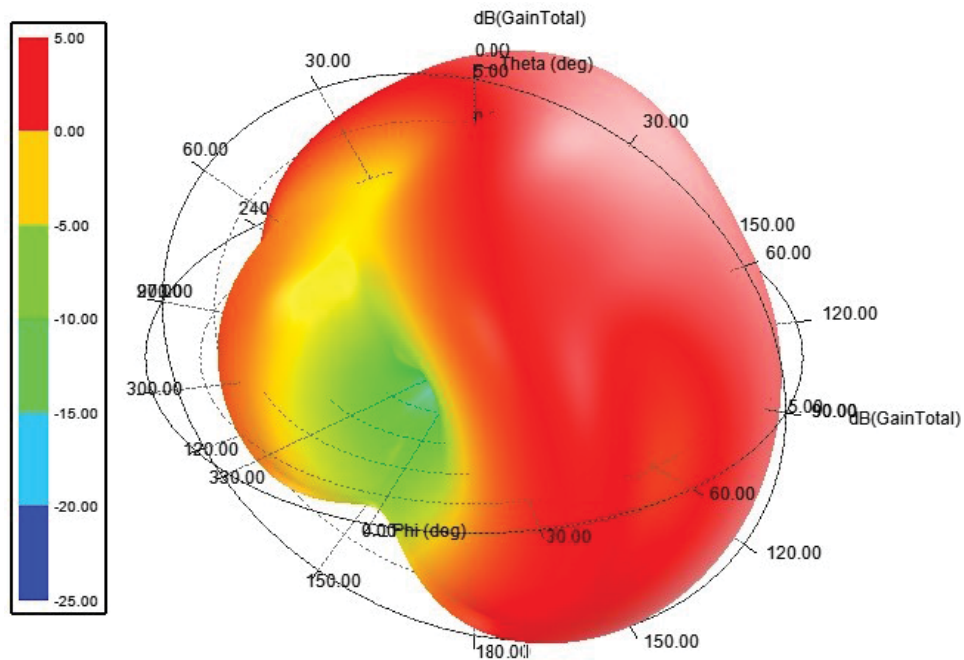
(a) Radiation patterns of antenna 3
