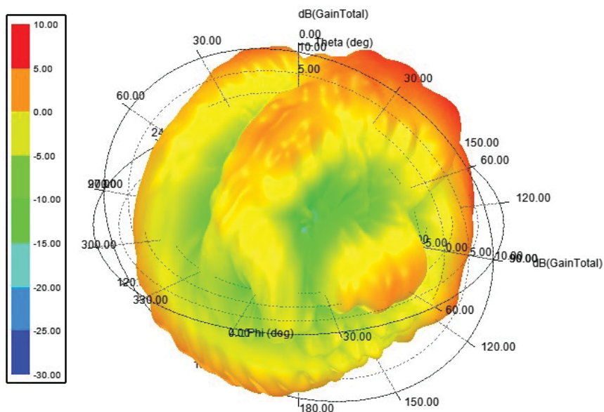
(a) 3D radiation patterns of antenna 5
