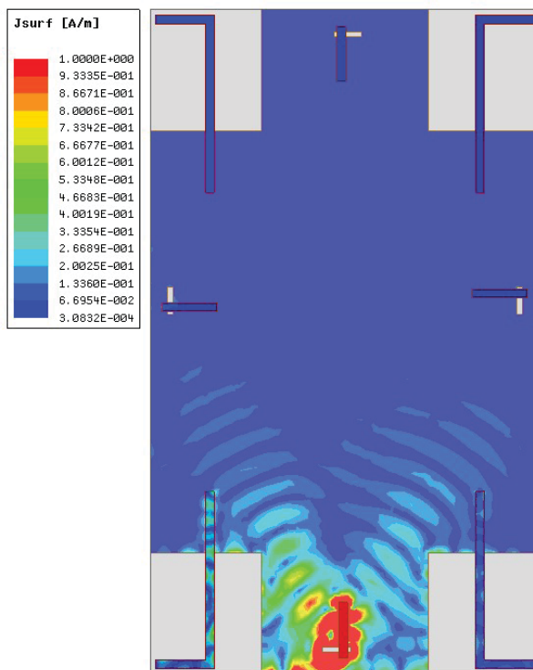
(b) Current distribution of 5G MIMO Antenna when antenna 5 is active
