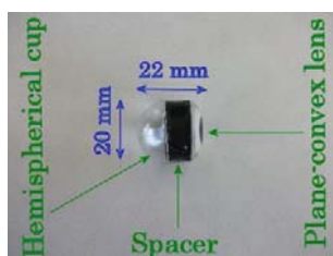
Fig. 7 Artificial eye
