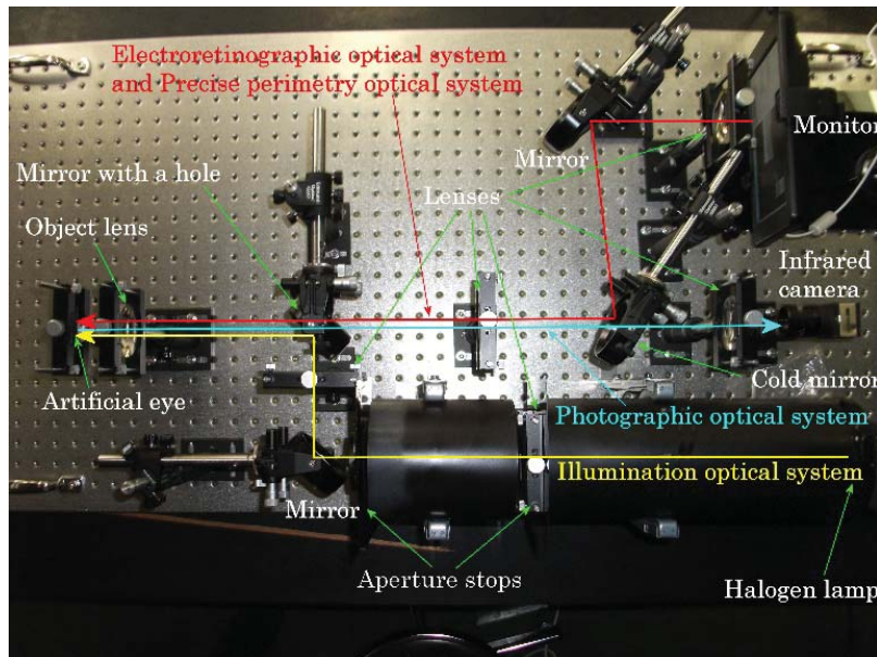
Fig. 6 Experimental device
