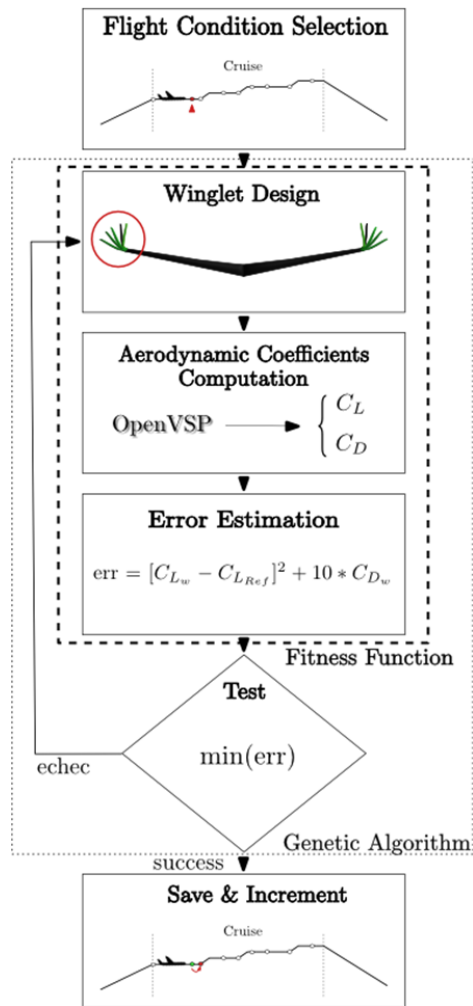
Fig. 7 Fitness function coupled with GA in charge of finding winglet geometry that optimizes aerodynamic coefficients characteristics of a wing for a selected flight condition
