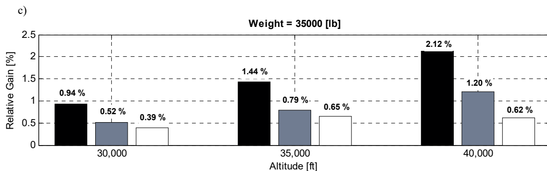
Fig. 10 Fuel gain obtained with an airplane equipped with an adaptive wing compared to fuel burn by an airplane equipped with the reference wing for several cruise simulations, and a fixed duration of 4 hours
