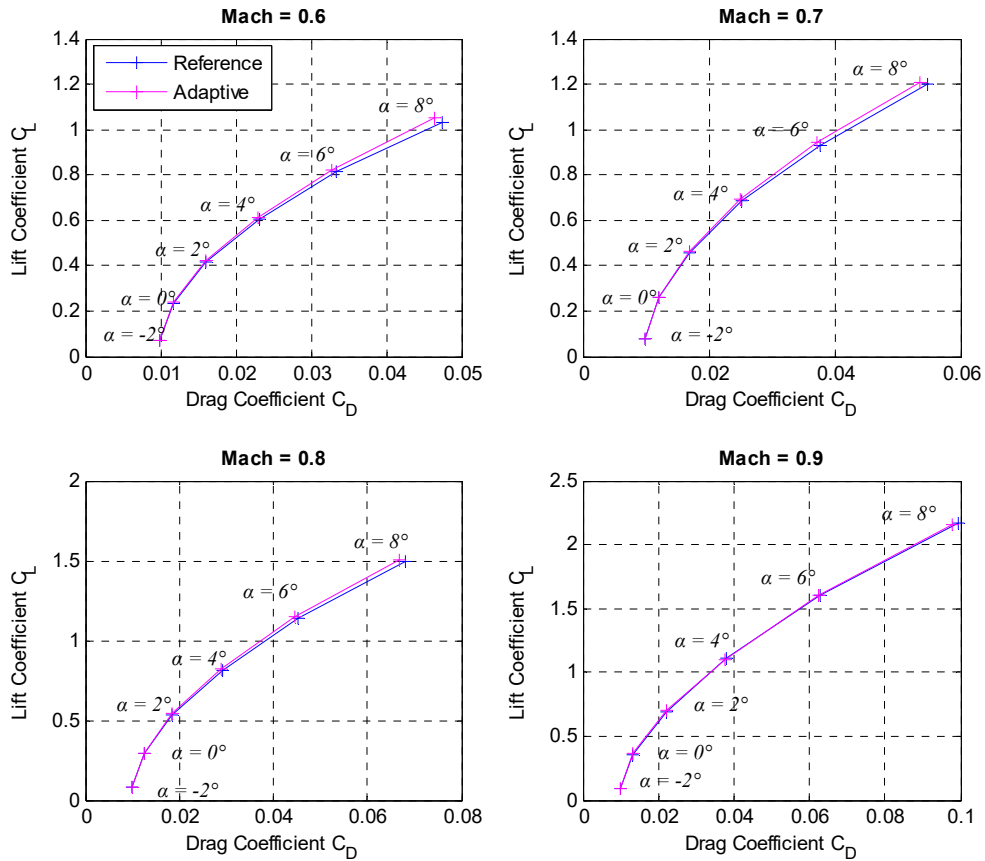
Fig. 8 Aerodynamic polar of the adaptive and the reference wing for Mach number 0.6 to 0.9
