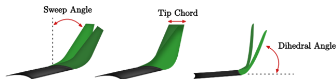
Fig. 6 Winglet degrees of freedom
