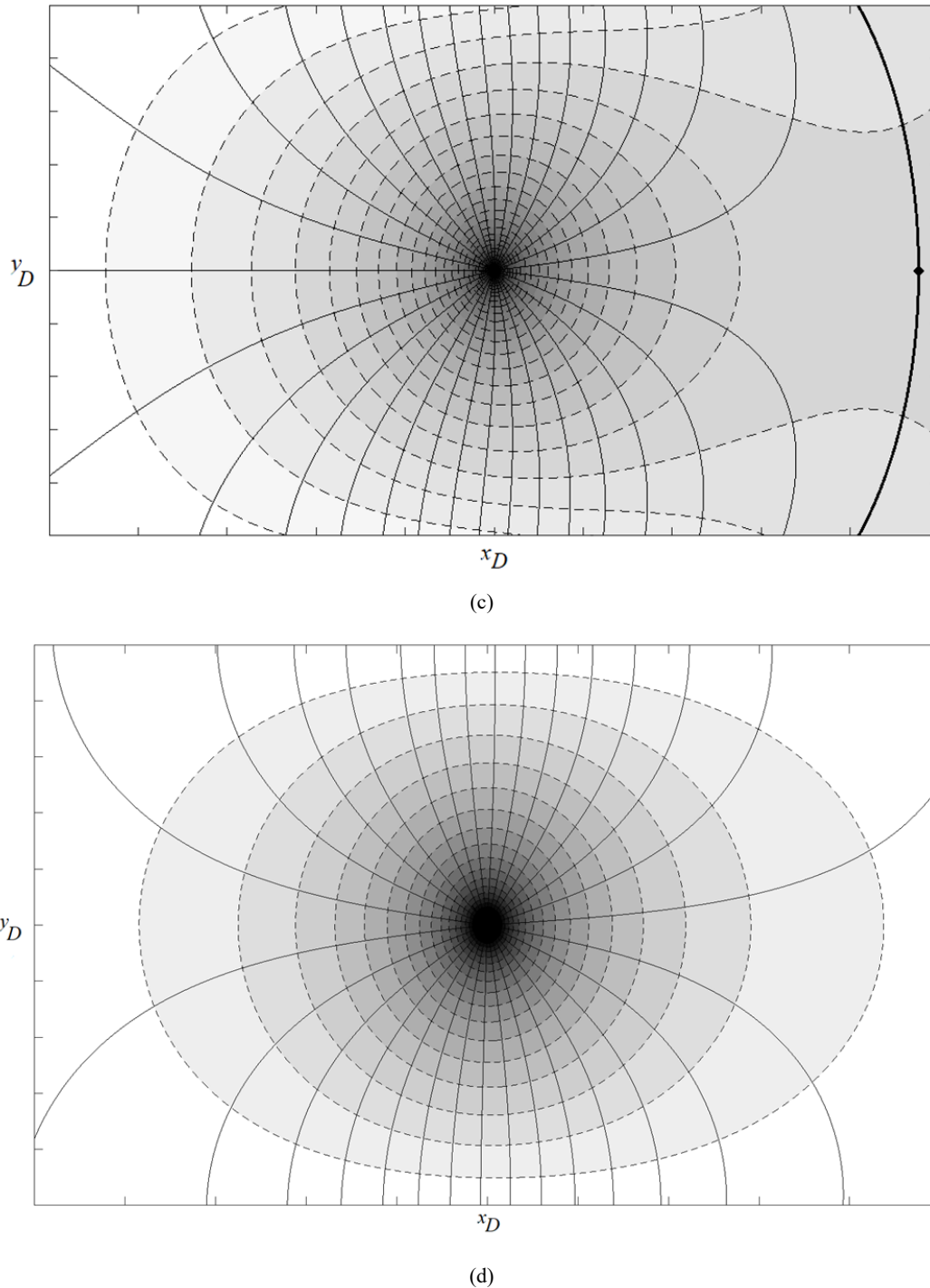
Fig. 2 Velocity potential and stream function for one well with extraction rate of 0.001 (a), 0.01 (b), 0.1 (c) and 1 (d) in a strip-shaped with constant head – constant head boundary ( \beta = 0 )
