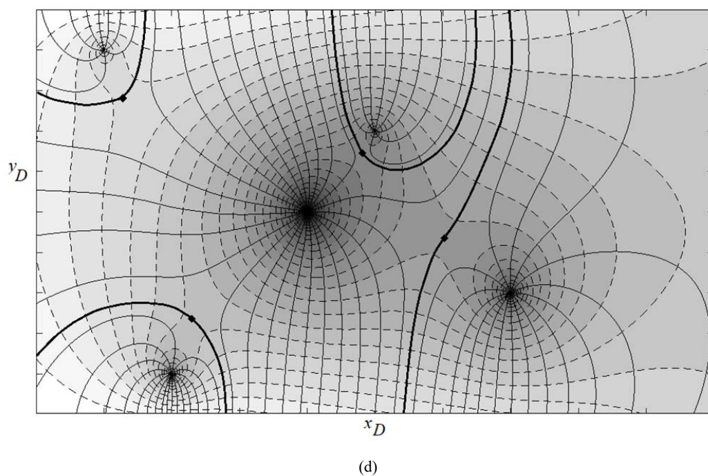
Fig. 3 Velocity potential and stream function for one (a), two (b), three (c) and five (d) wells in a strip-shaped with constant head – constant head boundary ( \beta = 0 )
