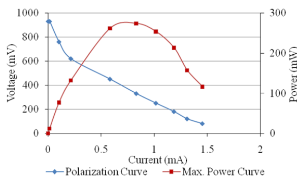
Fig. 5 Characteristics of cow dung battery
