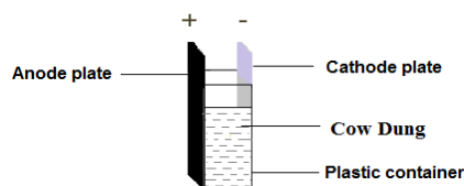
Fig. 1 Schematic representation of a single bio-voltaic cell
