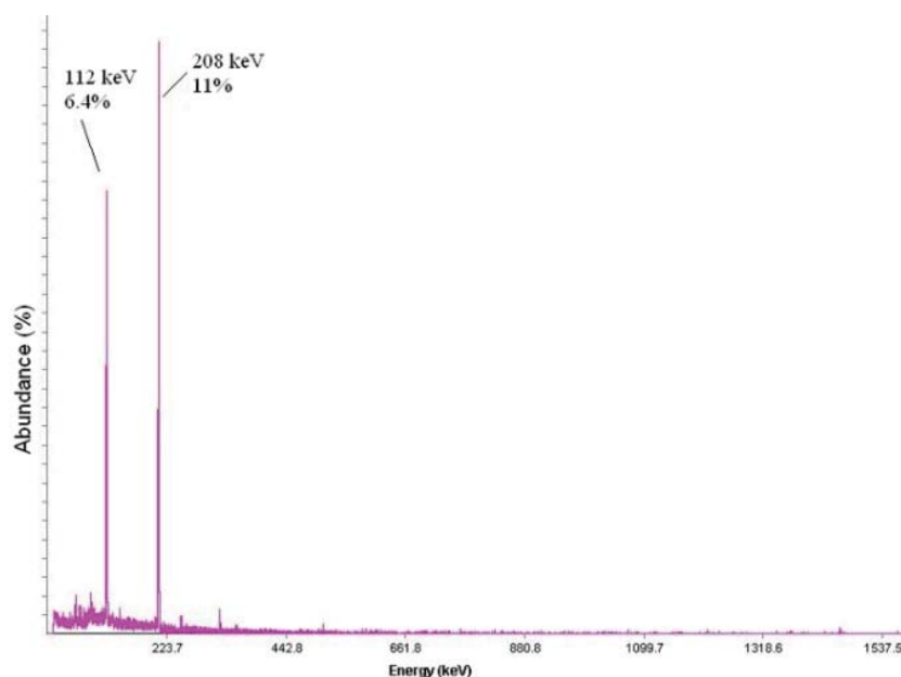
Fig. 1 HPGe spectrum of ^{177}\text{LuCl}_3
