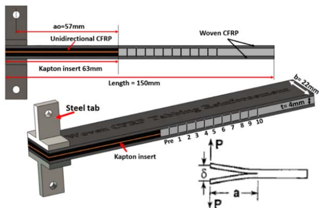
Fig. 3 Side view and 3D view of the DCB- Mode I test specimen showing the dimensions, the tabbing reinforcement and the propagation marks
