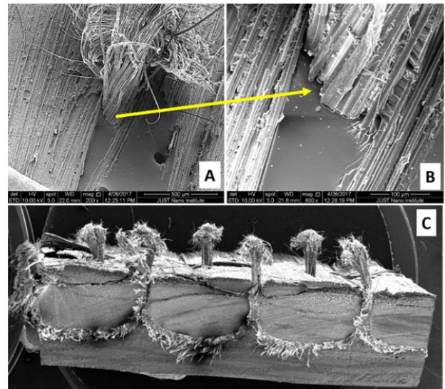
Fig. 9 SEM images of fractured sample stitched with Kevlar showing (A) A single Kevlar stitching thread with the epoxy matrix and carbon fibers (B) The adhesion between the thread's multi filaments and the epoxy (C) 3D view of the fractured sample
