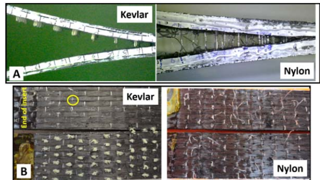
Fig. 8 Optical microscopic images of (A) Side view of samples stitched with Kevlar and nylon during the DCB test (B) Fractured surfaces of the same stitched samples
