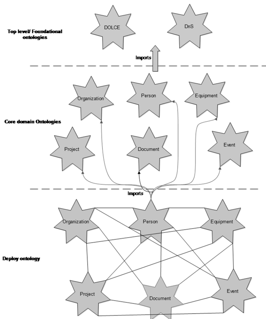
Fig. 2 R&D project ontology construction
