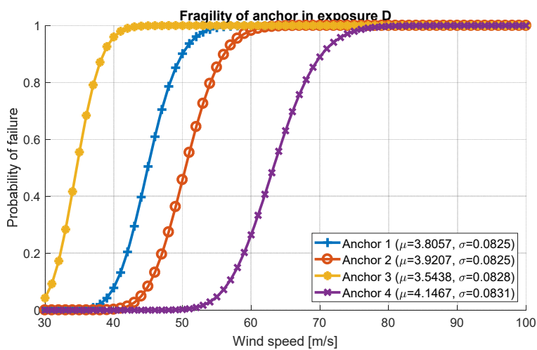
Fig. 8 Wind fragility of set Anchor (Exposure D)
