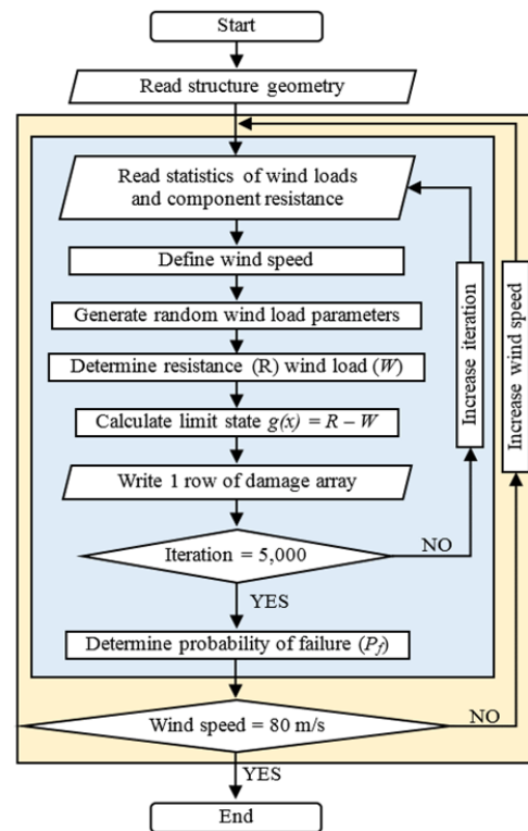
Fig. 5 Monte Carlo Simulation flowchart
