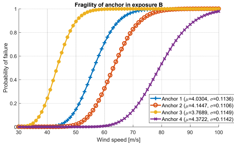
Fig. 6 Wind fragility of set Anchor (Exposure B)
