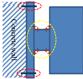
Fig. 4 Typical sign structure model in Korea
