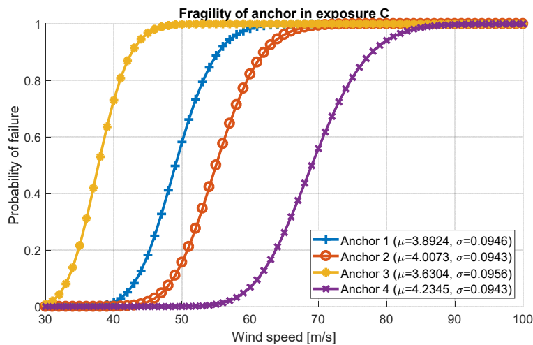
Fig. 7 Wind fragility of set Anchor (Exposure C)
