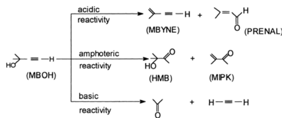
Fig. 1 Possible three pathways reactivity of MBOH [20], [21]
