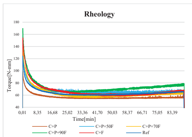
Fig. 3 Graphical evaluation of rheology measurements
