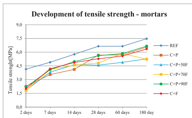
Fig. 7 Result of tensile strength after bending
