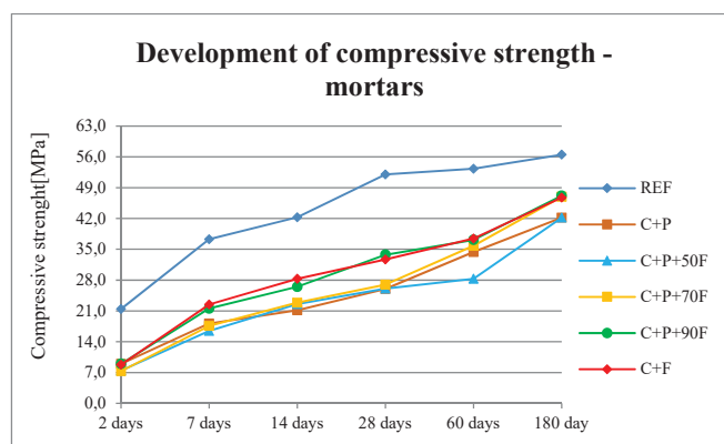
Fig. 6 Results of compressive strength testing
