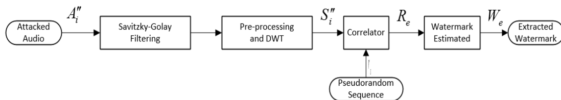
Fig. 2 Structure of extraction scheme
