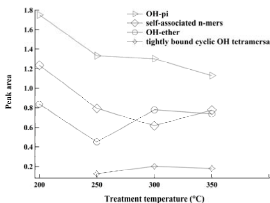
Fig. 3 Variation of hydrogen bond in the OH stretching region
