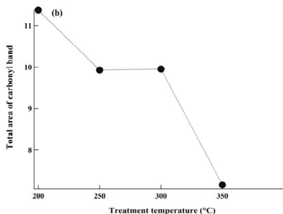
Fig. 4 (a) Variation in peak area of carboxylic acid and their derivatives and (b) variation of carbonyl band (1770, 1740, 1710, 1670 and 1650 \text{cm}^{-1} ) with varied treatment temperatures
