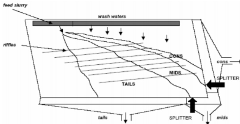
Fig. 5 Shaking table (Abols and Grady) [3]
