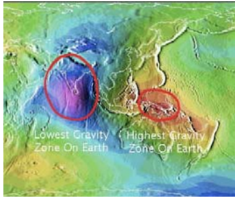
Fig. 3 Lowest and highest gravity zones on Earth [1]
