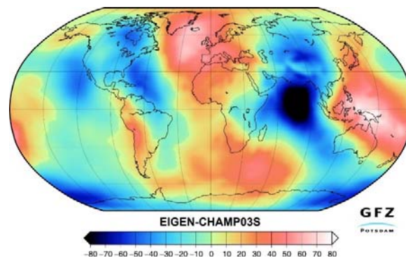
Fig. 2 Earth gravity anomaly map [1]
