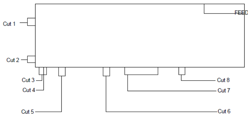
Fig. 8 Wilfley Table plane view and separated sample fraction collection (cut 1- 8)
