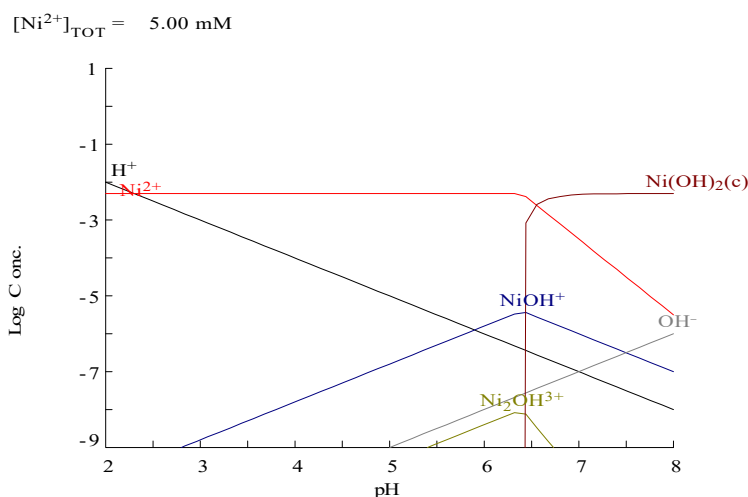
Fig. 6 Distribution diagrams of Ni(II) ( 5 \text{ mmol}\cdot\text{L}^{-1} ) in sulfate media using Medusa and Hydra programs [12]
