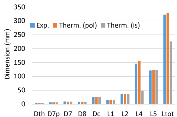
Fig. 8 Comparisons of dimensions for case 2 (CPM)
