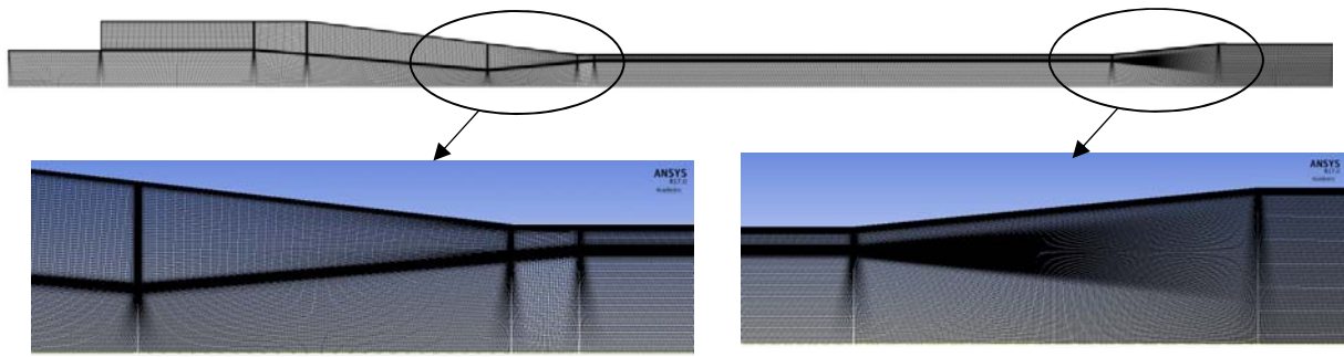
Fig. 4 Details of the mesh grid used in the CFD calculations for Case# 1 (CAM)
