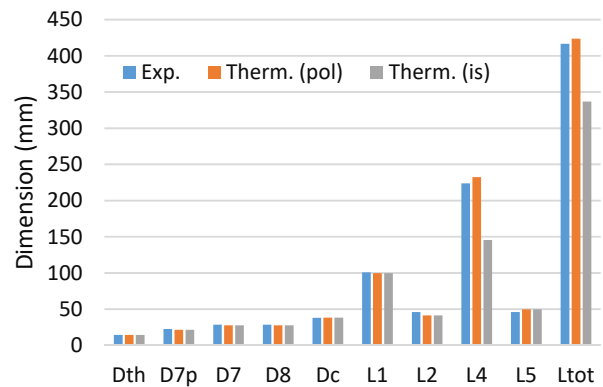
Fig. 7 Comparisons of dimensions for case 1 (CAM)
