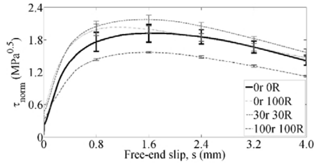
Fig. 10 Bond strength slip range
