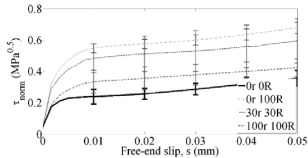
Fig. 8 Chemical adhesion slip range
