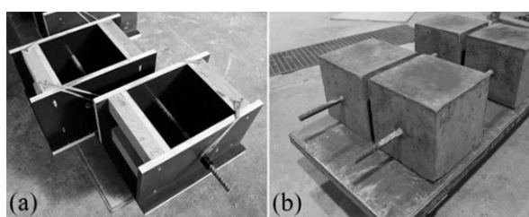
Fig. 2 (a) Formworks, (b) Hardened pull-out specimens
