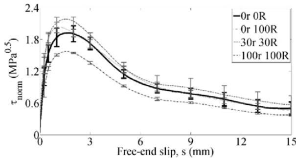
Fig. 7 Normalized bond stress/free-end slip curves
