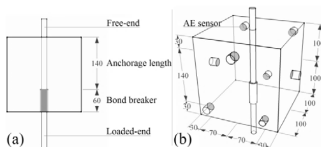
Fig. 3 (a) Interface design, (b) AE sensor distribution
