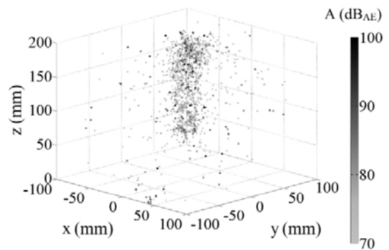
Fig. 11 Overview of the damage spread
