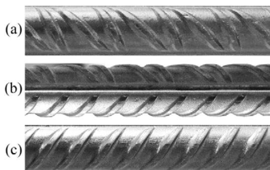
Fig. 1 Overview of the steel rebar rib patterns
