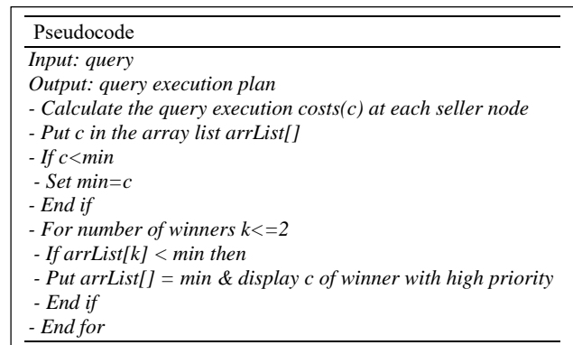
Fig. 9 Pseudocode of the proposed strategy
