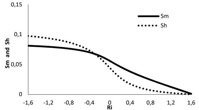
Fig. 2 Variation of stability functions vs Richardson number
