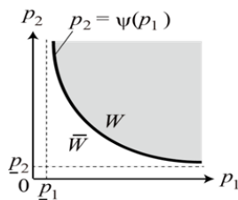
Fig. 2 Feasible region
