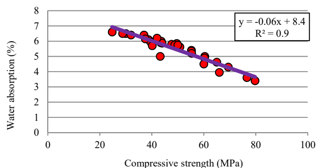
Fig. 12 Relationship between water absorption and compressive strength
