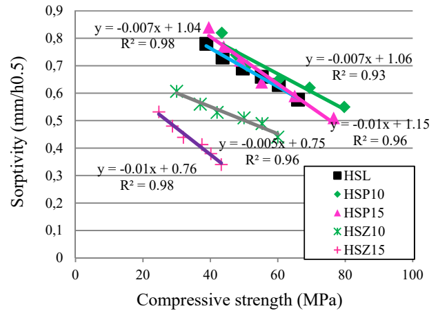
Fig. 16 Evaluation of sorptivity according to the compressive strength
