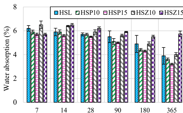
Fig. 9 Absorption after immersion (%) of studied HSSCCs
