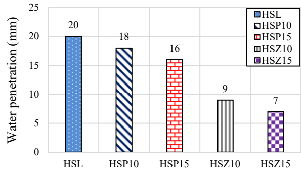
Fig. 17 Water penetration in the studied HSSCCs after 28 days of curing
