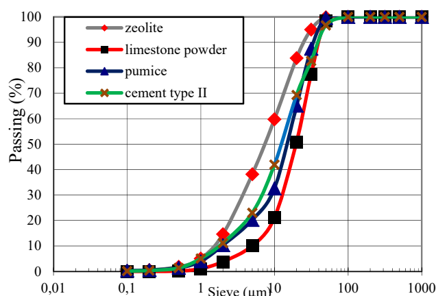
Fig. 1 Particle size distribution of fine materials
