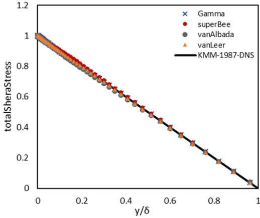
Fig. 1 Total shear stress for fully developed channel normalized by the wall shear velocity
