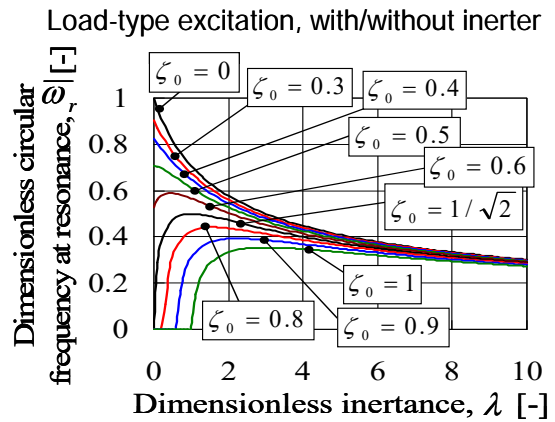
Fig. 6 Variation of the dimensionless circular frequency at resonance versus the dimensionless inertance, for various damping ratios
