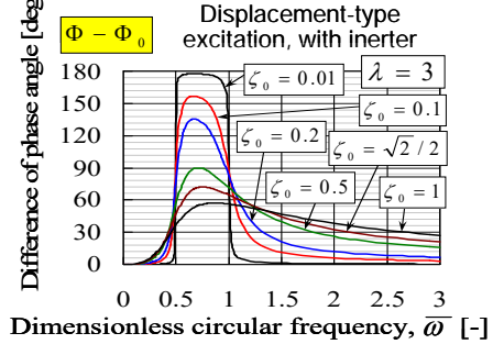
Fig. 15 Variation of the difference of phase angles versus the dimensionless circular frequency, for a fixed larger value of the dimensionless inertance, and various values of the damping ratio
