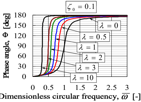
Fig. 12 Variation of the phase angle versus the dimensionless circular frequency, obtained under load-type excitation in the presence and absence of the inerter, for a fixed value of the damping ratio
