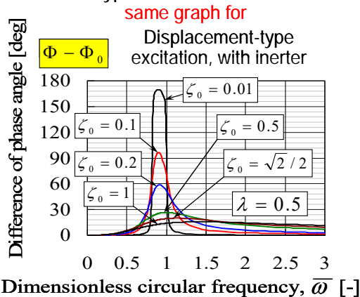
Fig. 14 Variation of the difference of phase angles versus the dimensionless circular frequency, for a fixed smaller value of the dimensionless inertance, and various values of the damping ratio
