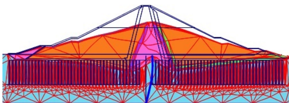
Fig. 8 Deformed mesh with stone columns
