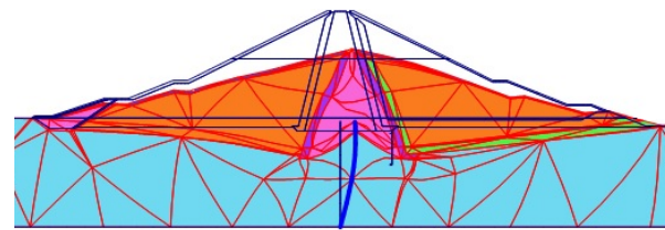
Extreme total displacement 3.86m (Displacement scaled up 5 times)
