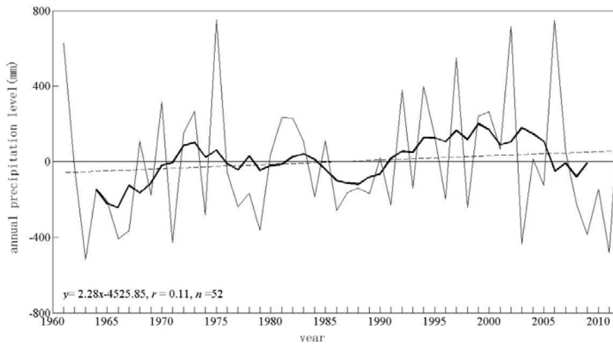
Fig. 1 Anomaly Variation of Precipitation
