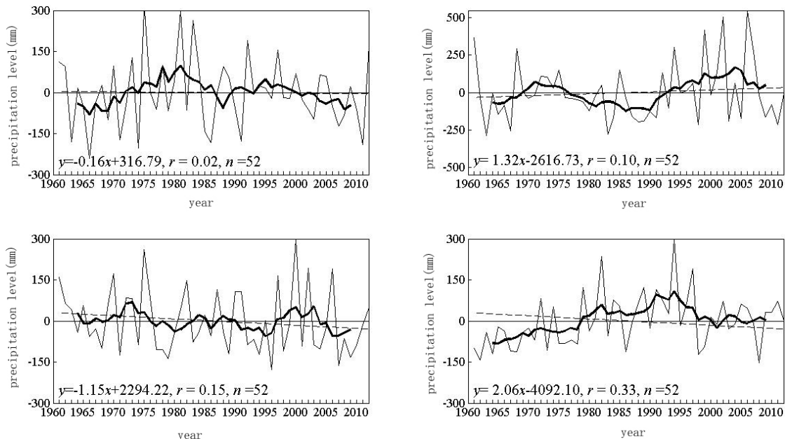
Fig. 2 Anomaly Variation of Seasonal Precipitation
