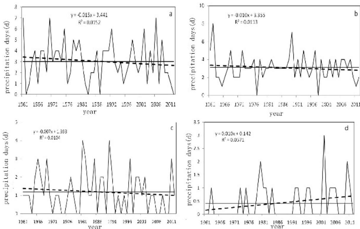
Fig. 8 Seasonal Extreme Precipitation Event Variation
