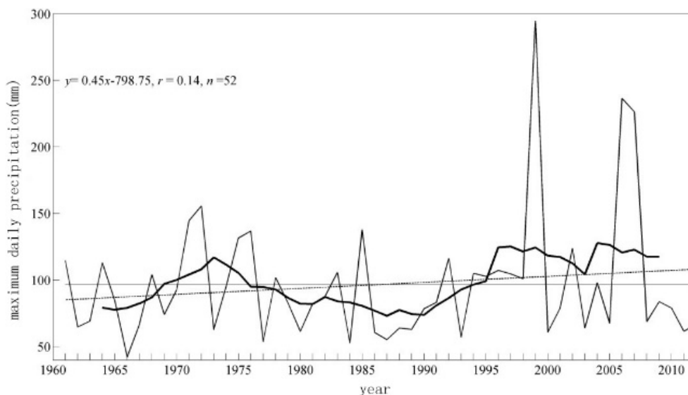
Fig. 9 Maximum Daily Precipitation Variation from 1961 to 2012
