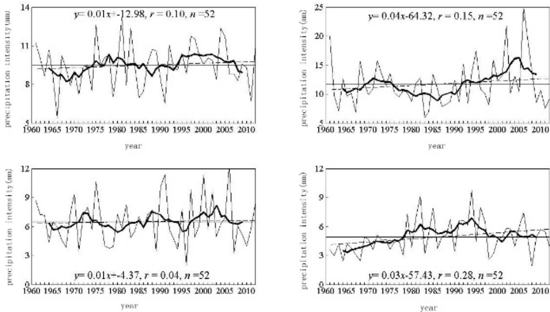
Fig. 6 Seasonal Precipitation Intensity Variation
