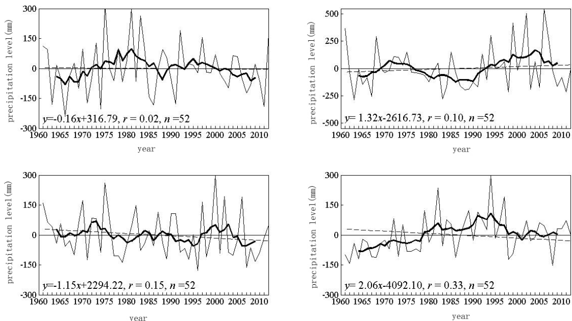
Fig. 2 Anomaly Variation of Seasonal Precipitation
