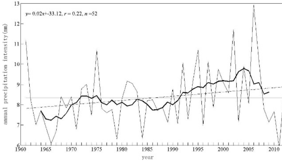
Fig. 5 Annual Precipitation Intensity Variation
