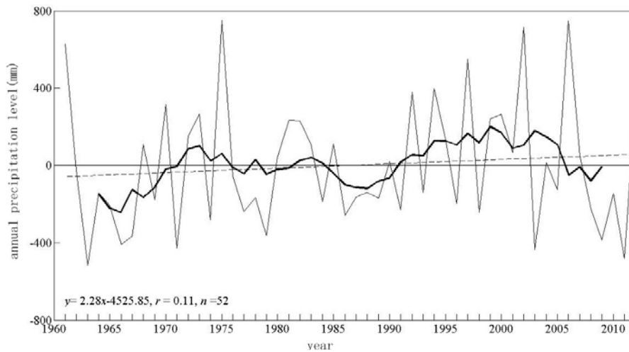
Fig. 1 Anomaly Variation of Precipitation
