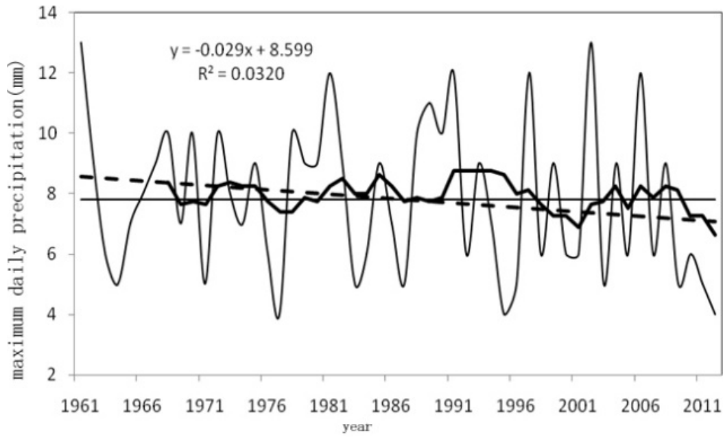
Fig. 7 Yearly Extreme Precipitation Event Variation
