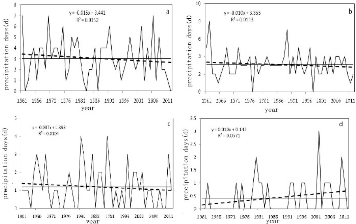
Fig. 8 Seasonal Extreme Precipitation Event Variation
