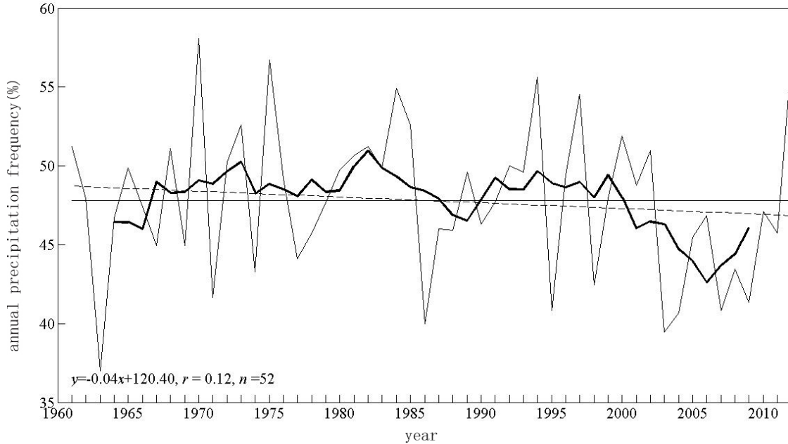
Fig.3 Yearly Precipitation Frequency Variation
