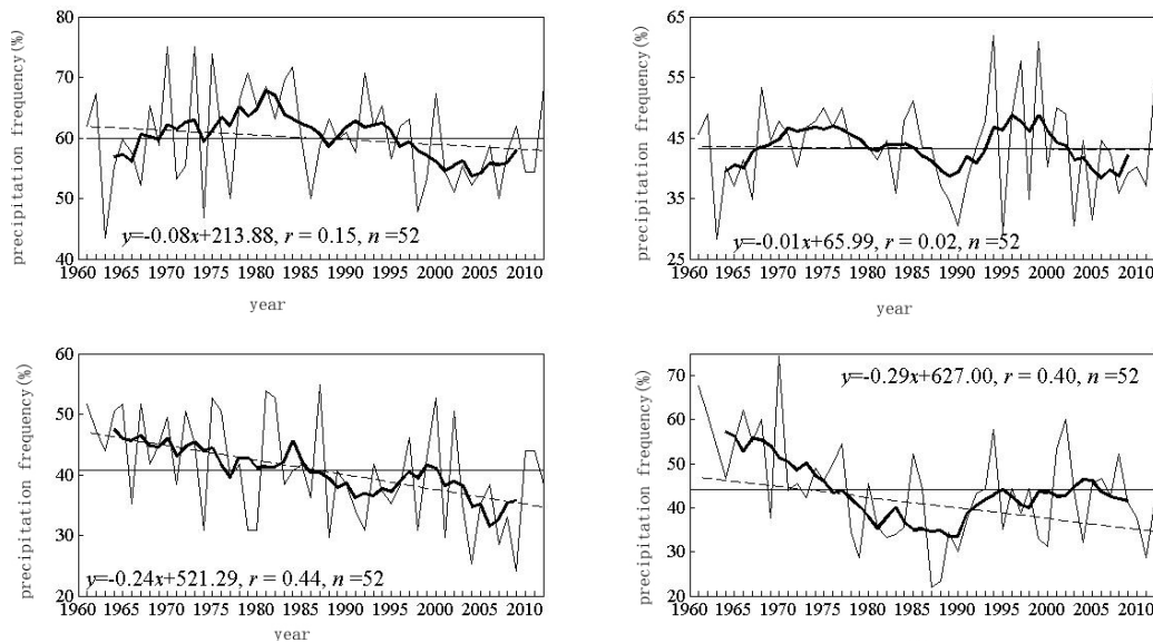
Fig. 4 Seasonal Precipitation Frequency Variation of Chenzhou
