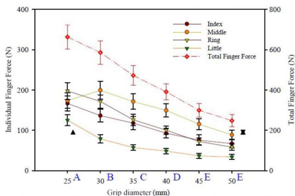
Fig. 2 Gripping force for various grip diameters [10]
