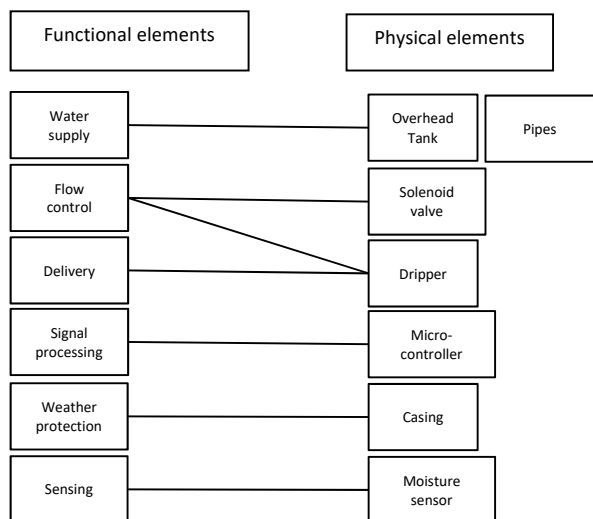
Fig. 6 Slot Modular Architecture of SMCS
