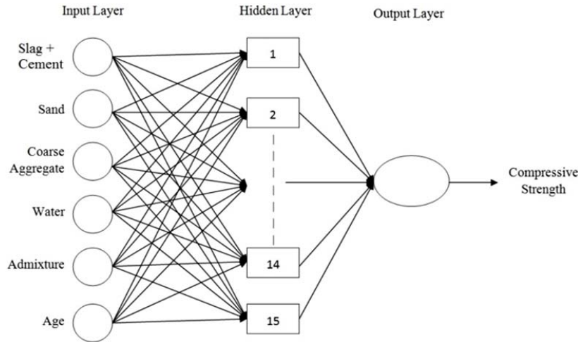
Fig. 2 ANN structure for the proposed research work
