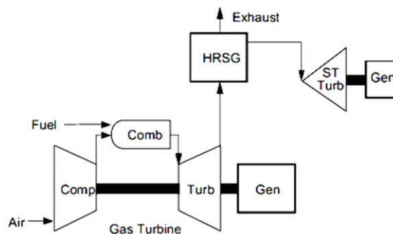
Fig. 1 Component diagram of the combined gas turbine cycle
