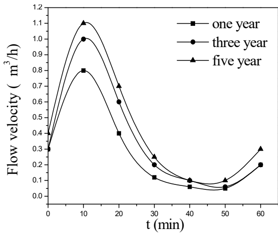
Fig. 3 The flow velocity under different return periods
