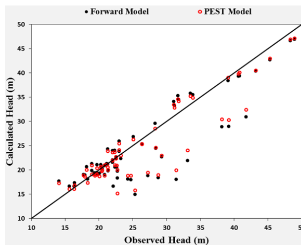
Fig. 3 Comparison of the calculated and observed heads for the Forward and PEST models
