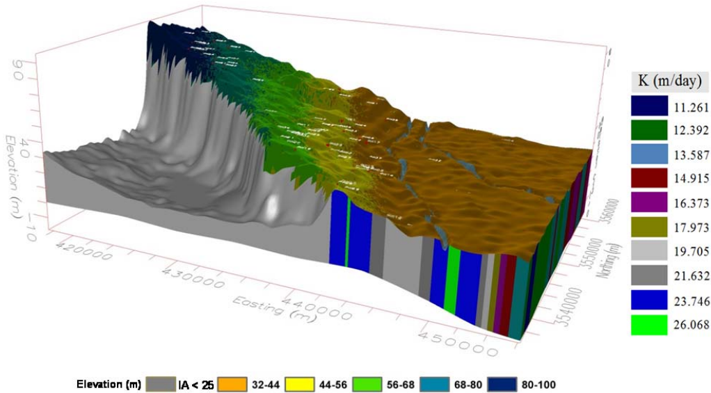
Fig. 5 3D-view of the PEST Model-One Unconfined Aquifer-One Heterogeneous Soil Layer without interface soil layer
