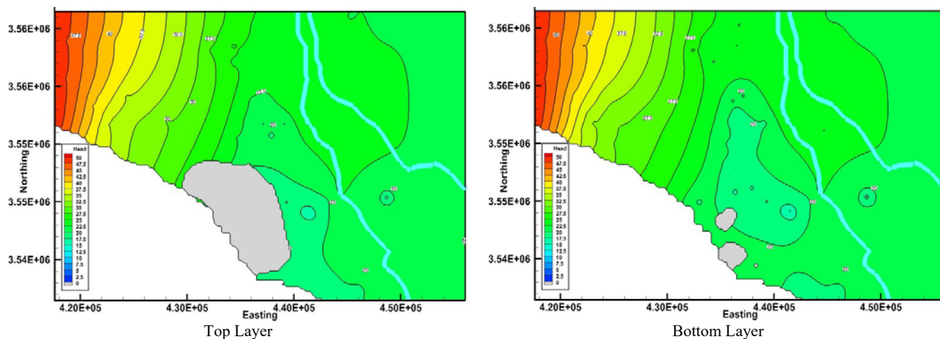
(a) PEST Model-One Unconfined Aquifer-Two Heterogeneous Soil Layers
