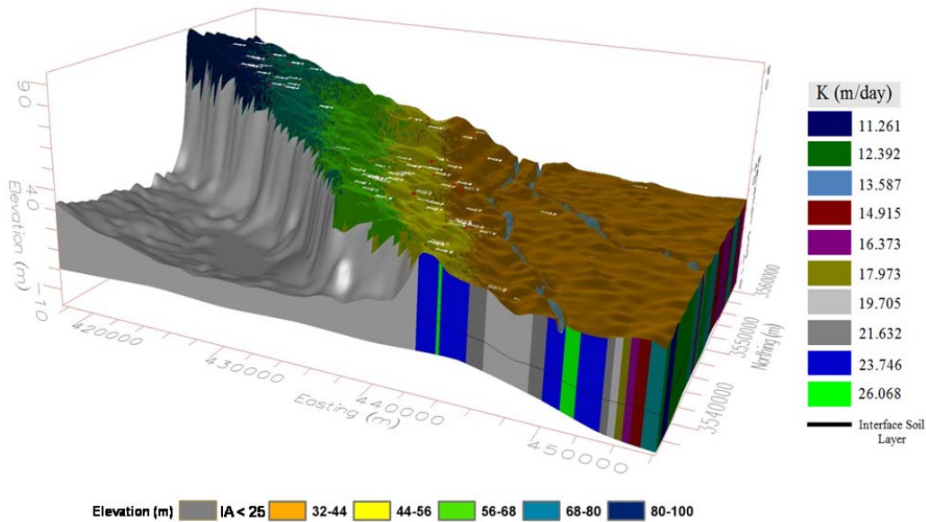
Fig. 4 3D-view of the PEST Model-One Unconfined Aquifer-Two Heterogeneous Soil Layers separated by interface soil layer
