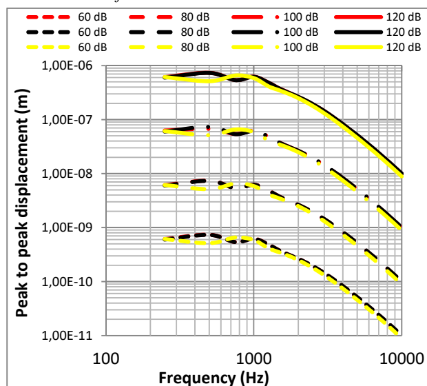
Fig. 3 Peak to peak displacement of stapes footplate, Healthy ME, Silicon, Titanium
