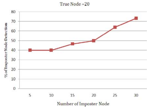
Fig. 6 Detection of imposter node in Case-2
