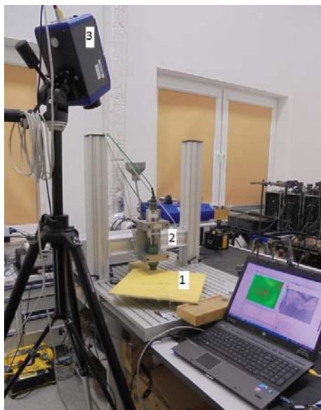
Fig. 2 Experimental set-up (1- sample, 2- ultrasound generator, 3- IR camera)
