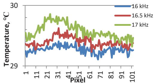
Fig. 5 Temperature signal over defect D2 for different ultrasonic frequencies
