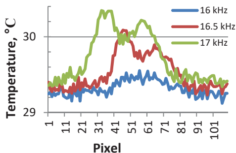
Fig. 4 Temperature signal over defect D1 for different ultrasonic frequencies
